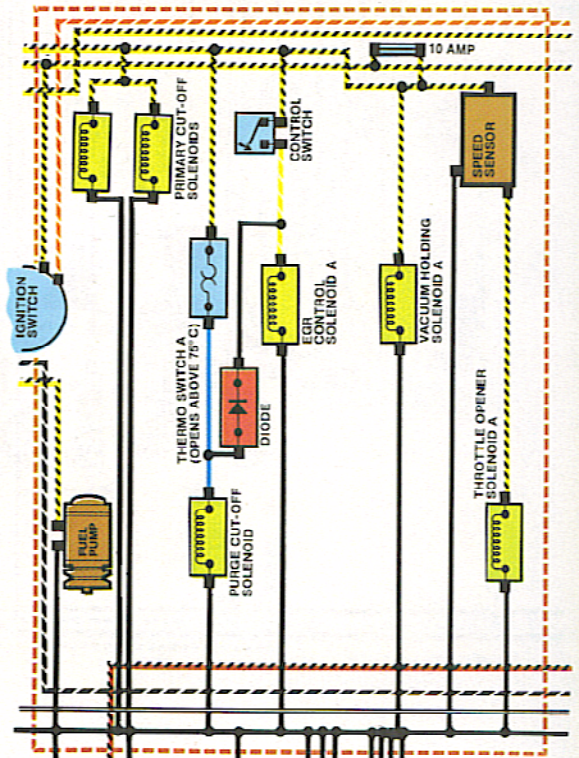
49-State & High Altitude Sedan
