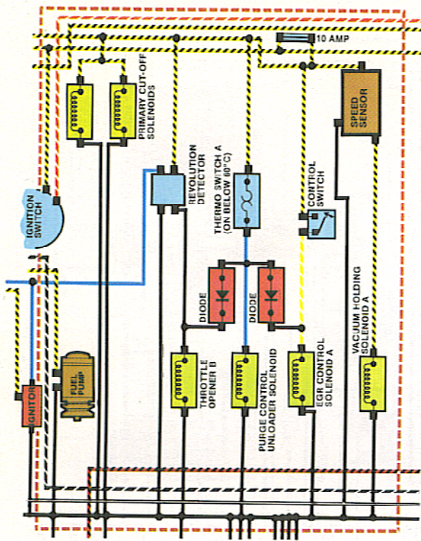
49-State & High Altitude Hatchback
